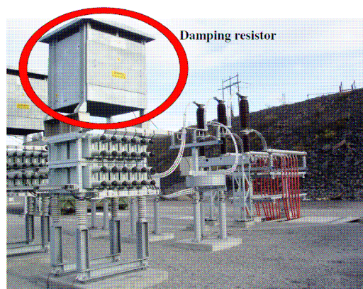
Picture 1. 12 th harmonic filter with damping resistor
