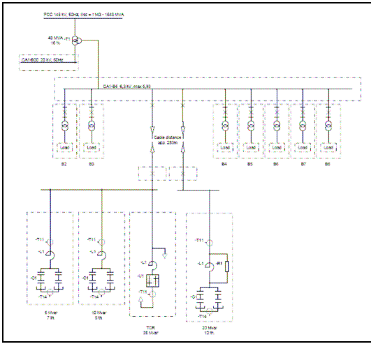
Figure 1. SVC, single-line diagram
